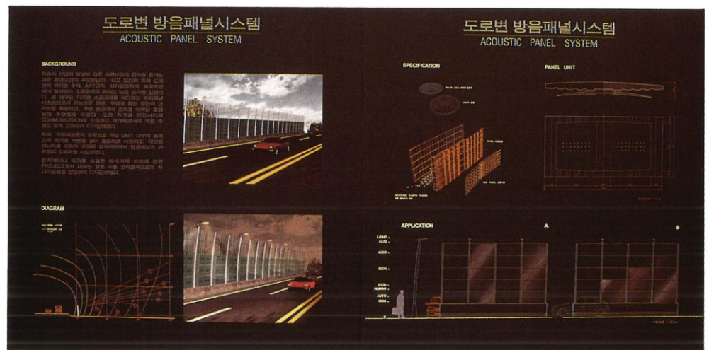
환경처장관상 도로변 방음패널 시스템 조태형 · 양영완 PRIZE OF THE MINISTER OF ENVIRONMENT ACOUSTIC PANEL SYSTEM CHO, TAI-HYUNG · YANG, YOUNG-WAN
