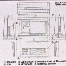
1. SPEAKER 2. LCD SCREEN 3. PRINTER PORT 4. 8mm VCR 5. FDD 6. KEY BOARD 7. CONTROL BUTTON
